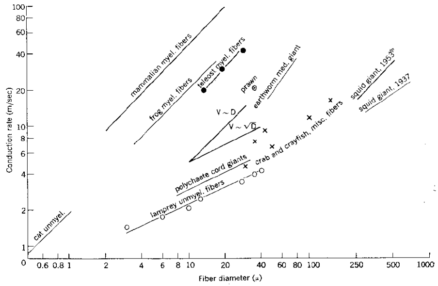
Figure 3.12. Velocity of nerve impulse conduction as a function of fiber diameter. A wide assortment of animals and preparations is compared. Where lines are not drawn the data for fibers of the same type but different diameter are not available.
