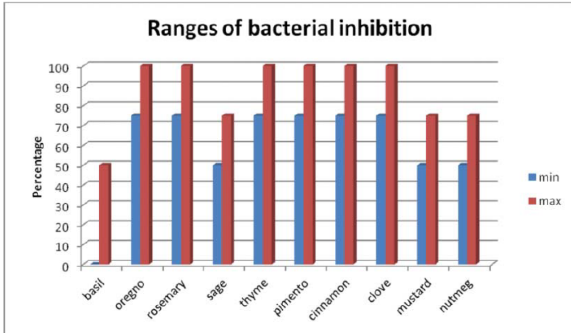
Figure 2. Ranges of bacterial inhibition data for different spices (adapted from Naidu, 2000; Ceylan and Fung, 2004; Holley and Patel, 2005).
