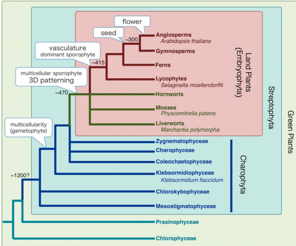
Fig. 1. Phylogenetic relationships between major groups of extant green plants.
