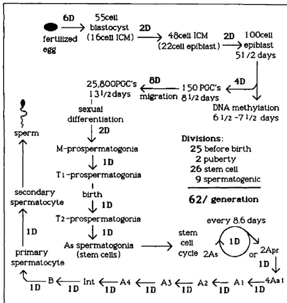
Fig. 5. Mouse male germ cell divisions. Spermatogenesis begins at 6 days. Stem cell divisions occur every 8.6 days. The stem cell division resulting in mature sperm at 9 months (274 days) occurred in the cycle ending 43 days earlier, and there have been (274-43-6)/8.6 = 26 stem cell divisions.
