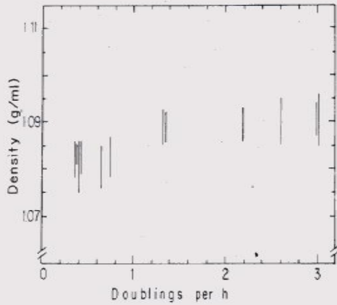
Fig. 6. Mean cell density of E. coli B/r H266 as a function of growth rate. Vertical bars indicate the position of cell bands as estimated by optical inspection of either self-generated or preformed gradients centrifuged at 20 to 24°C. From Woldring et al. , 1981.
