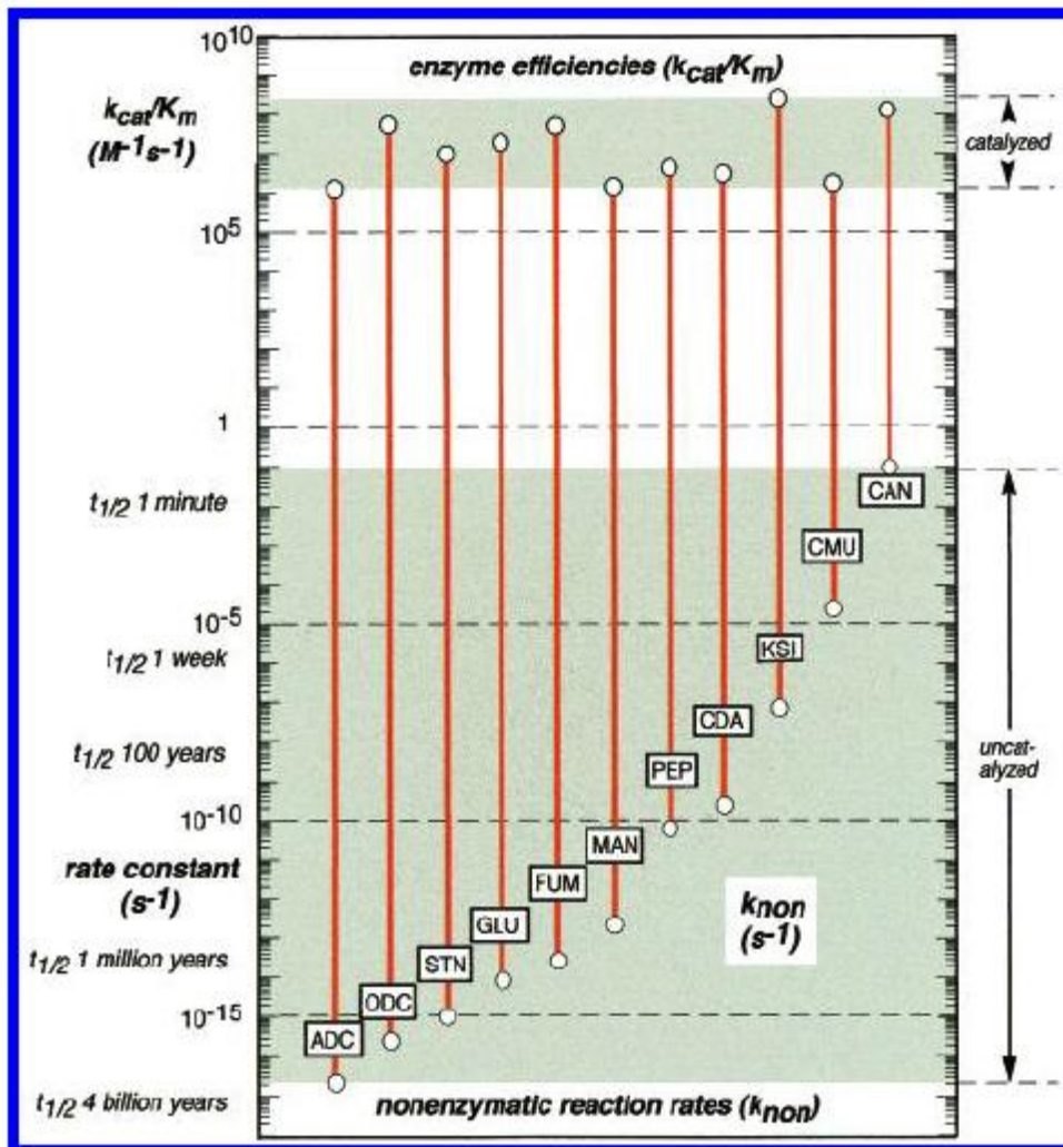
FIGURE 6. Logarithmic scale of k_{cat}/K_m and k_{non} values for some representative reactions at 25 °C. The length of each vertical bar represents transition-state affinity or catalytic proficiency (its reciprocal). For abbreviations and references, see Figure 5.
