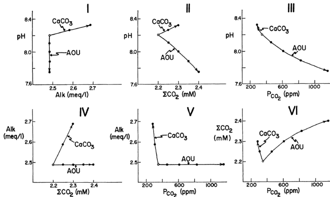
FIG. 2. The AOU and carbonate dissolution vectors on six two-parameter coordinates. The distance between two connected dots shows the change occurred by \Delta\text{CO}_2 of 0.050 mM either by AOU or carbonate dissolution (shown by \text{CaCO}_3 ). Carbonate alkalinity is expressed by Alk. Roman numerals correspond to the parameter combinations in the text.
