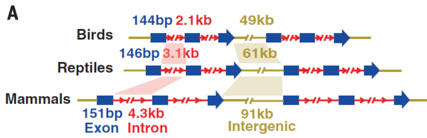
Fig. 2. Genome reduction and conservation in birds. (A) Comparison of average size of introns, exons, and intergenic regions within avian, reptilian, and mammalian genomes. (B) Synteny plot and large segmental deletions
