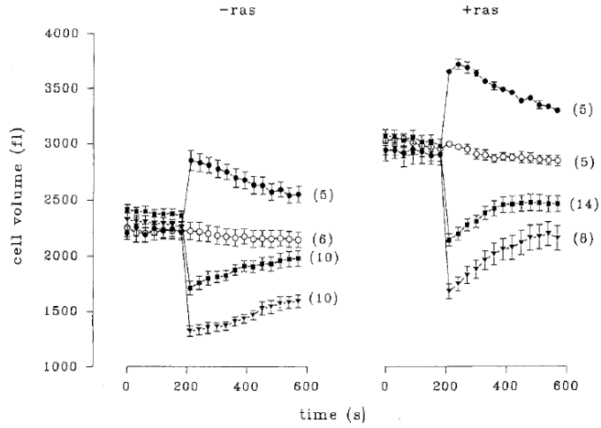
Fig. 3. Cell volume regulation of NIH 3T3 fibroblasts not expressing the ras oncogene ( -ras, left ) and of the same cells expressing the ras oncogene ( +ras, right ). The cell volume is plotted versus the time of incubation. At 180 s, extracellular osmolarity has been either decreased by reduction of extracellular NaCl by 35 mmol/l ( closed circles ), or increased by addition of 50 mmol/l NaCl ( closed squares ) or 100 mmol/l NaCl ( closed triangles ). The open circles refer to cells exposed to isotonic extracellular fluid. Arithmetic means \pm SEM, numbers in brackets indicate number of experiments
